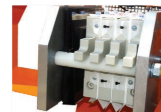
Filter chambers with airbag
